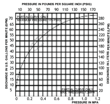
Nominal Discharge Curve
